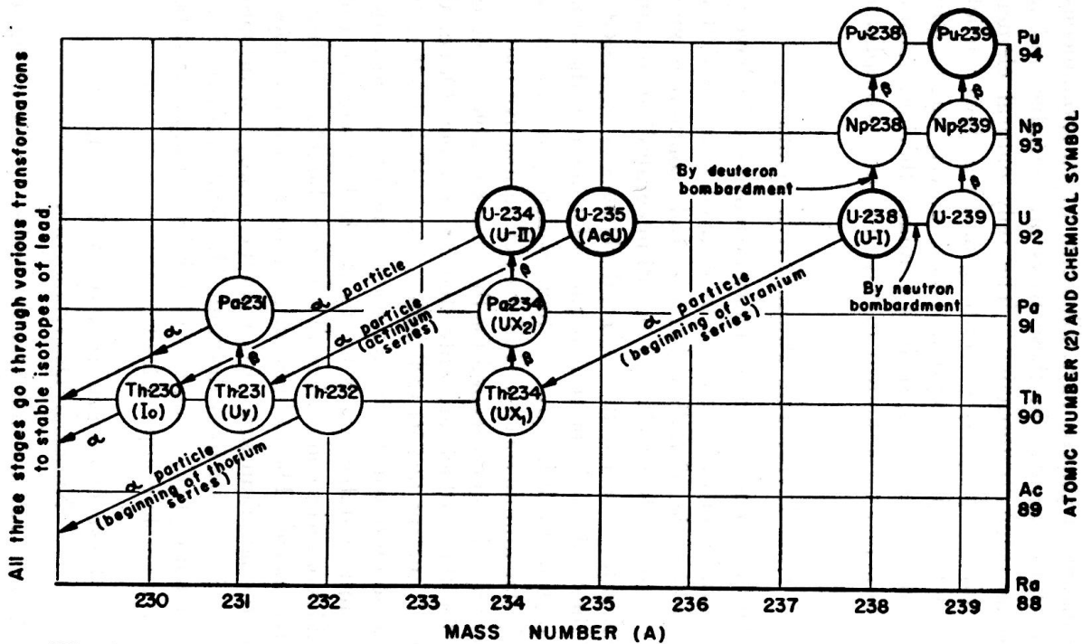
The beginnings of the three natural radioactive series and the new transuranic elements, neptunium and plutonium.
